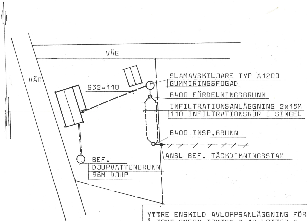
SITUATIONSPLAN 1:500
