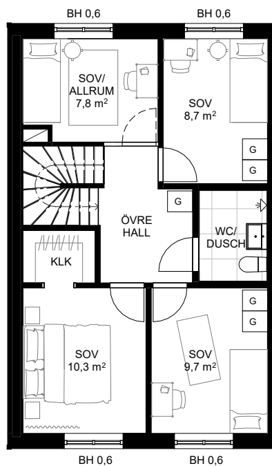
Mellanplan
