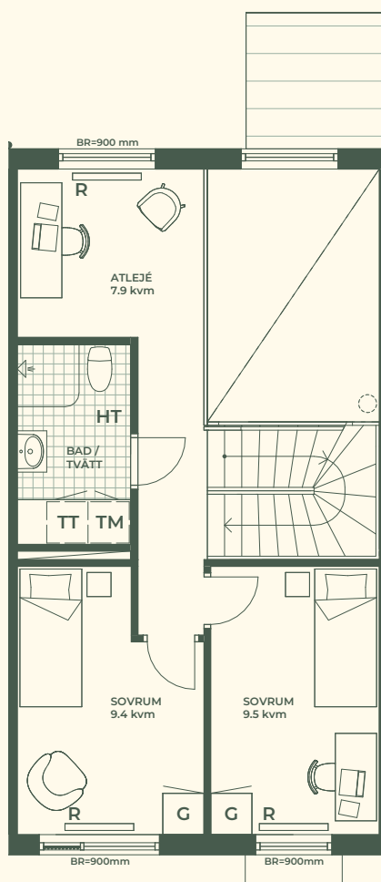
PLAN 2 RH = ca 2.5 m
