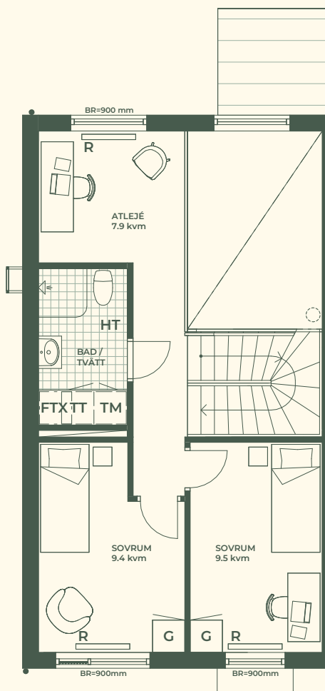
PLAN 2 RH = ca 2.5 m
