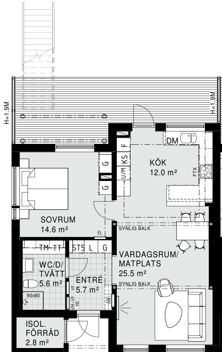
PLAN 1
