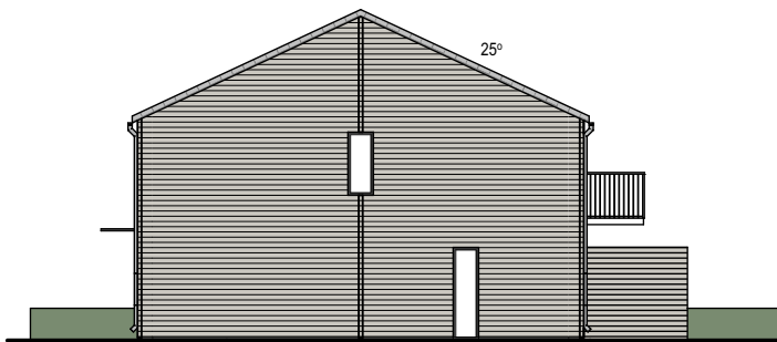
FASAD GAVEL
