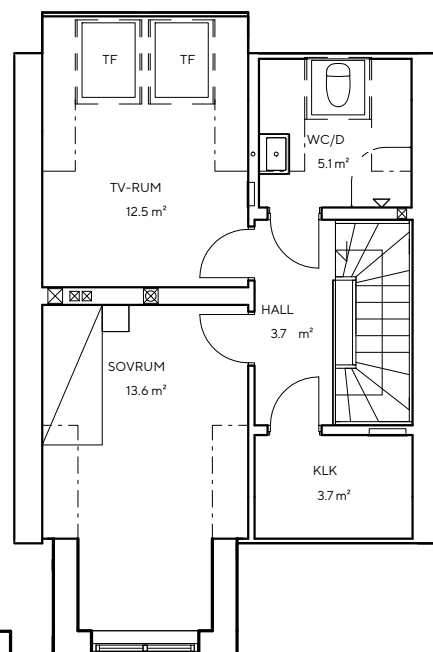
Plan 3 – 41,7 kvm
