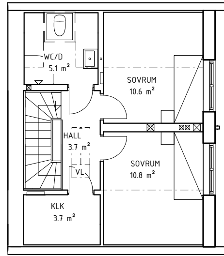
Plan 3 – 41,7 kvm
