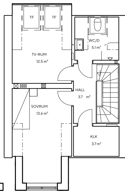
Plan 3 – 41,7 kvm
