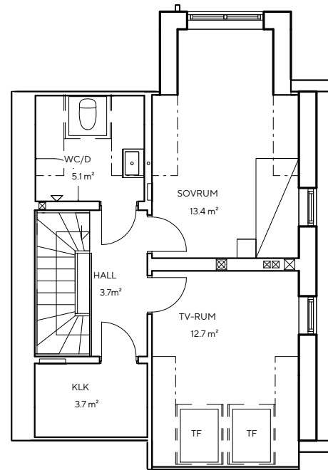
Plan 3 – 41,7 kvm
