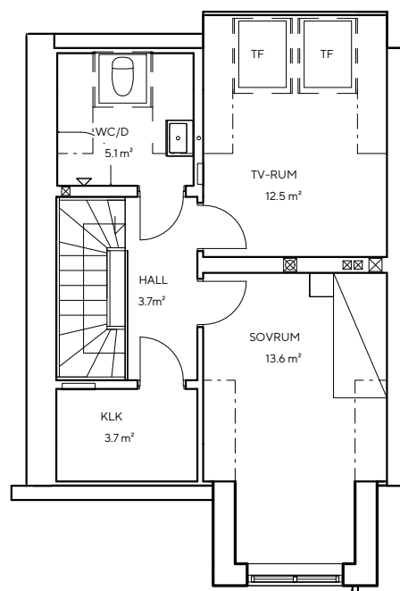
Plan 3 – 41,7 kvm
