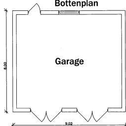
Bottenplan
