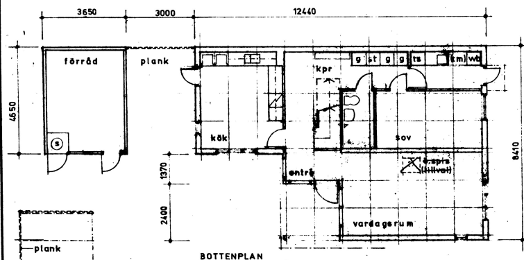
BOTTENPLAN
