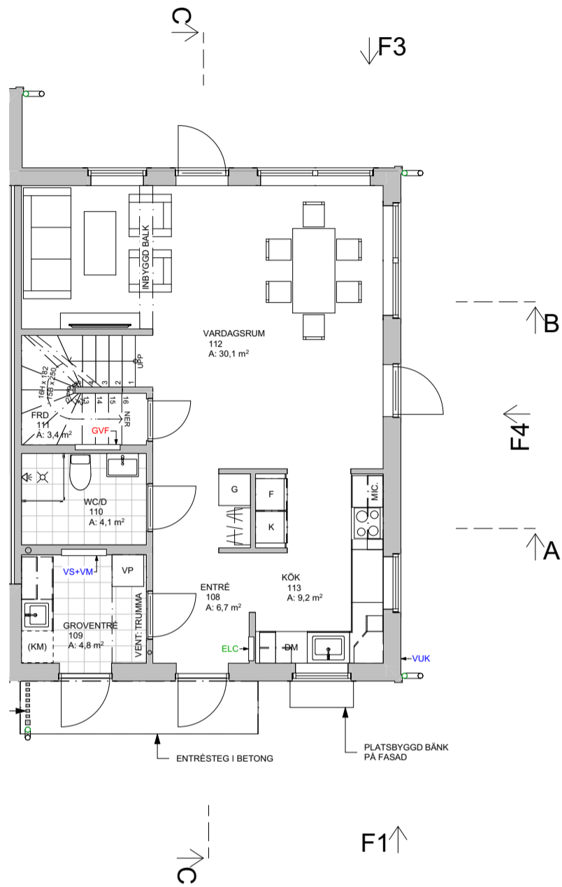
PLAN 1
