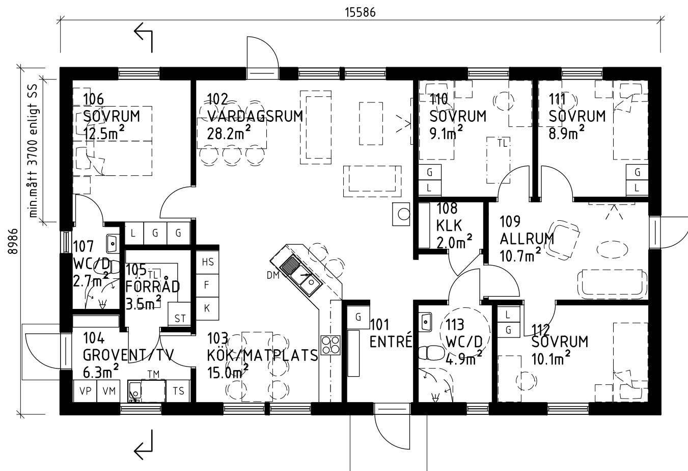
PLAN 140m 2 (BTA)
