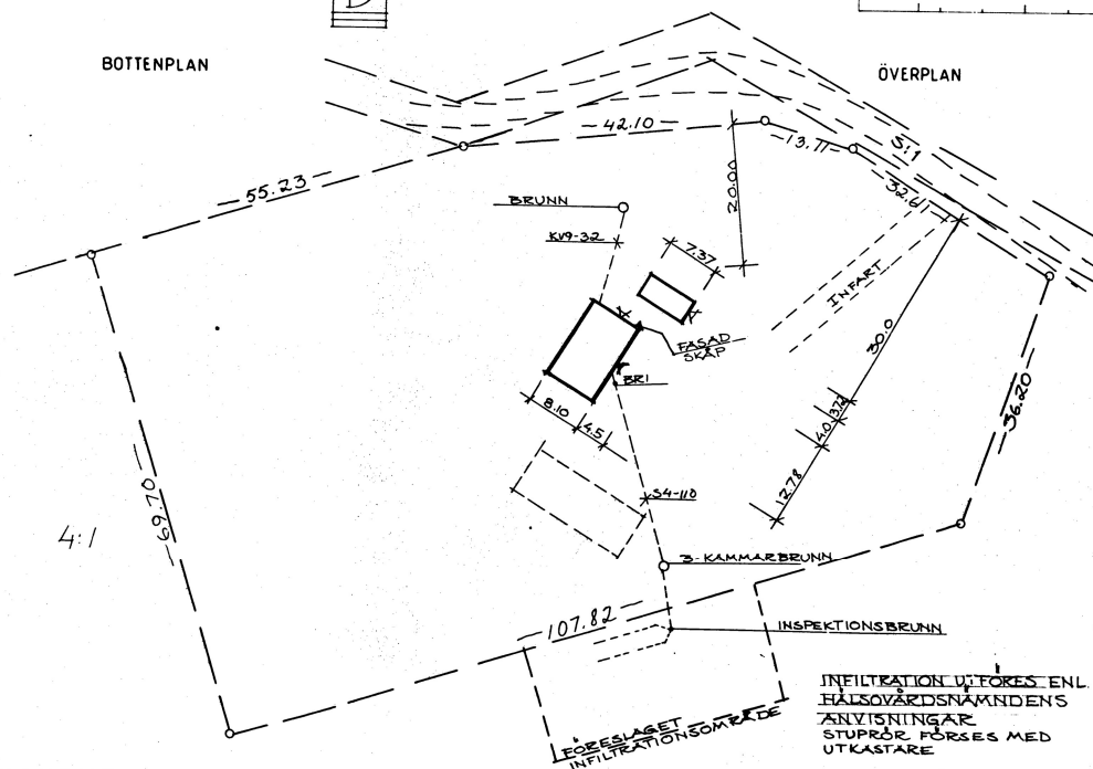
SITUATIONSPLAN 1:500
