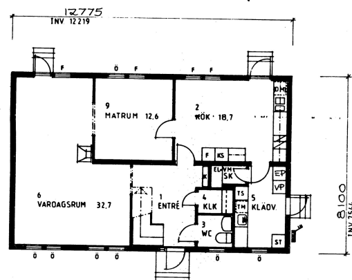
BOTTENPLAN
