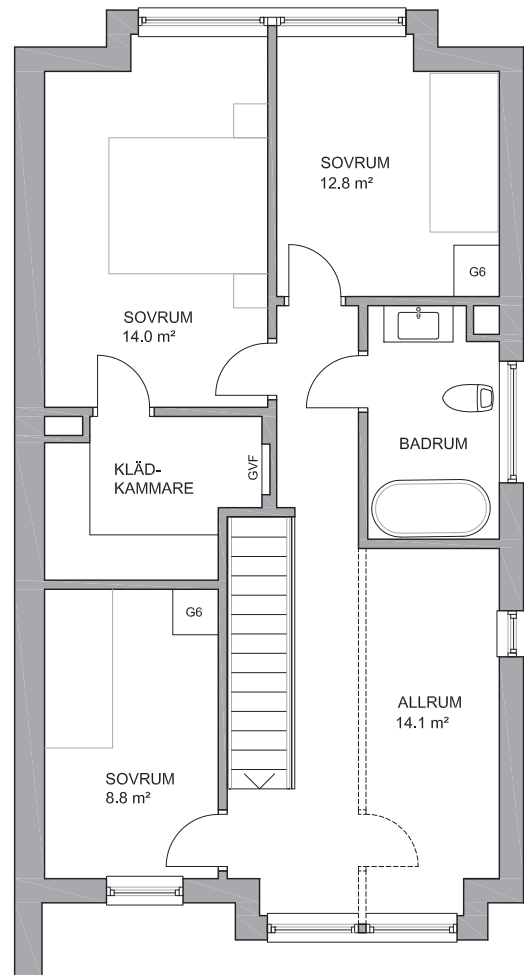
PLAN 2
