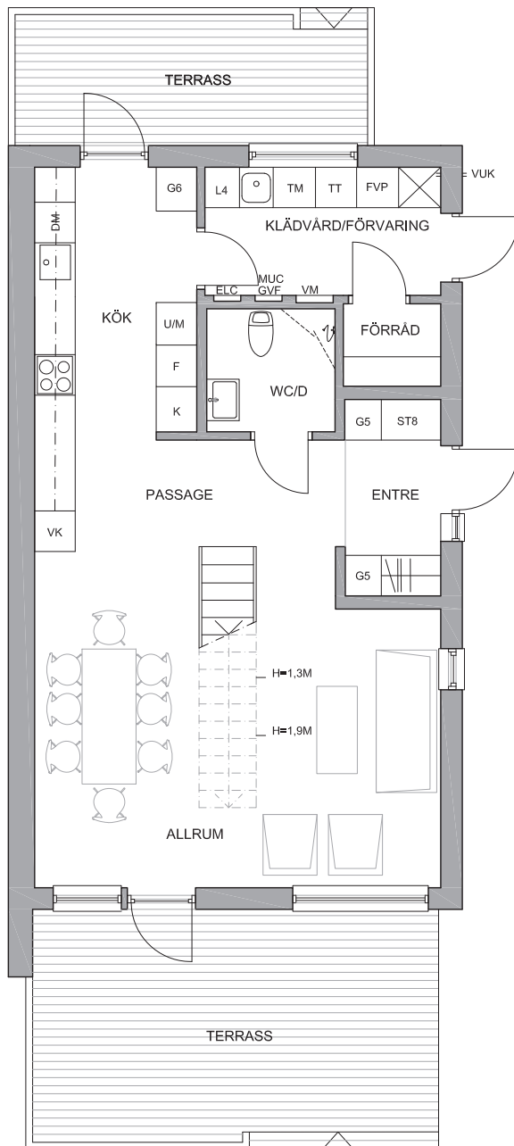
PLAN 1
