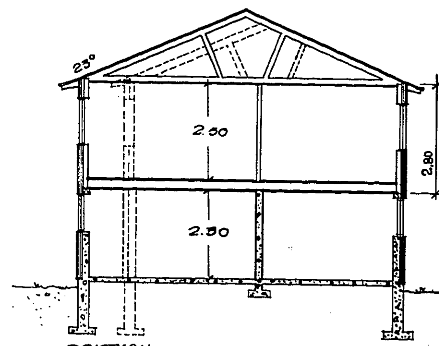
SECTION
