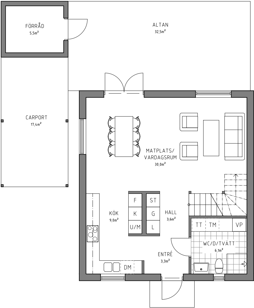
ENTRÉPLAN BOA: 56,0m²
