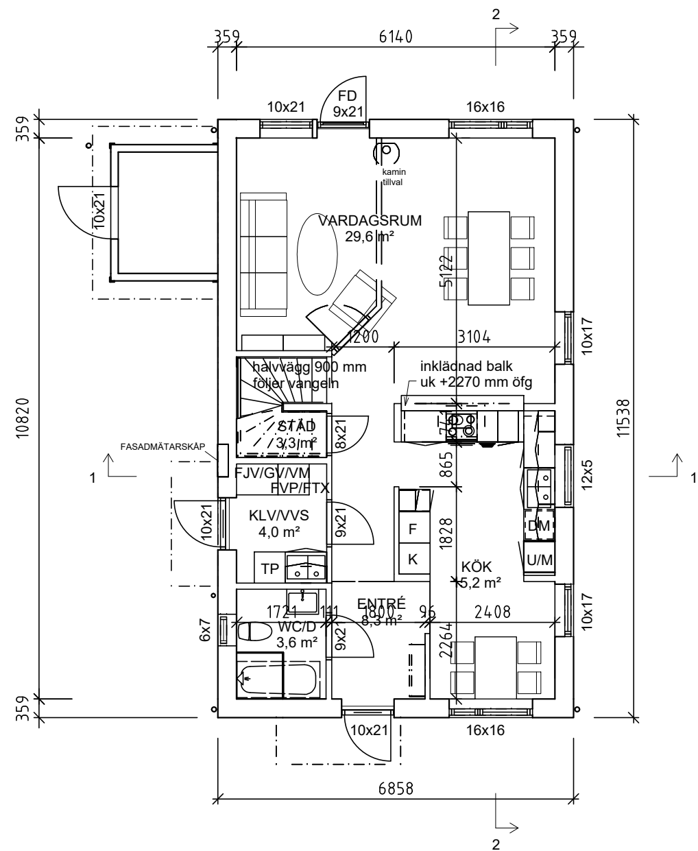
PLANVY PLAN 1 1:100 (A1)
