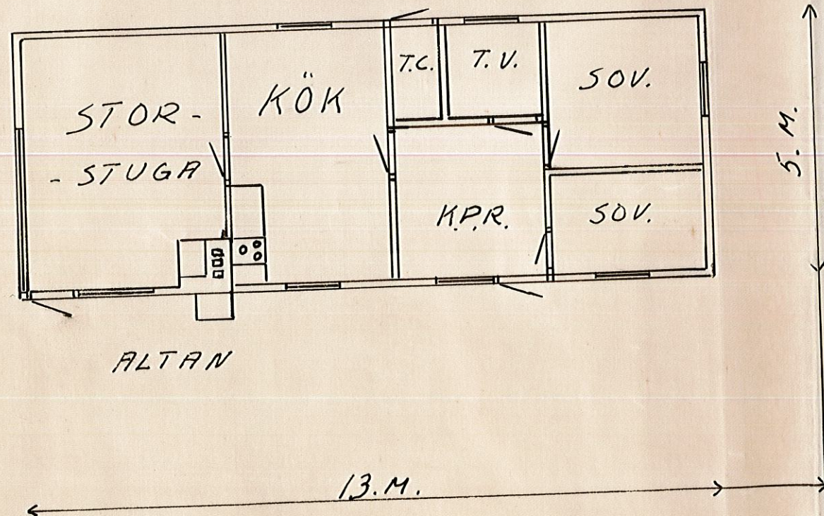
PLAN, 1: 100.
